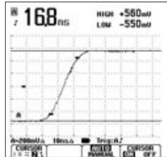
Figure 5: Fluke 124 measuring rise time automatically
