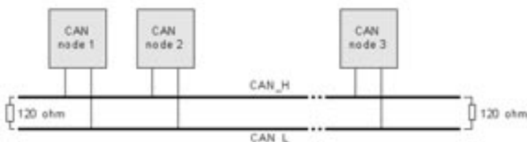
Figure 1. Two-wire CAN architecture
