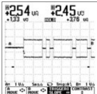
Figure 4. Changing the time-base allows you to zoom in and analyze signal details
