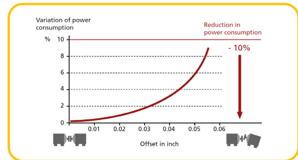
Power consumption in relation to offset. Courtesy of © ICI PLC
