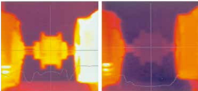
Thermography showing coupling overheating (left)
