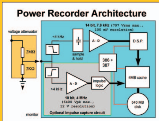
Figure 3. Sampling system architecture.
