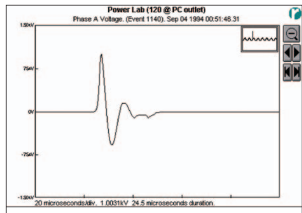
Figure 2 provides a look at the same capture as seen using high-speed analog-to-digital sampling techniques at rates of 1-MHz or more using Full Disclosure technology. The waveform that could provide the key to power problem analysis is clearly visible.
