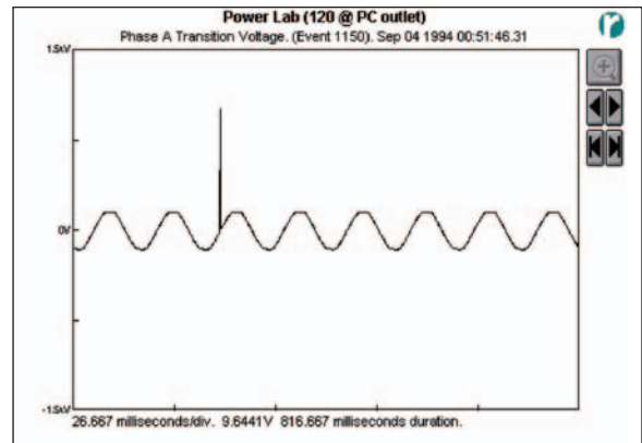
Figure 1 illustrates a peak detect impulse capture. When set at a sampling rate of 8 kHz, which permits capture of transients and impulses down to 130-msec duration, it is adequate for capturing power factor capacitor switching transients but not fast enough for recording high-speed impulses that occur inside facilities due to loads (motors, etc.) turning on and off.
