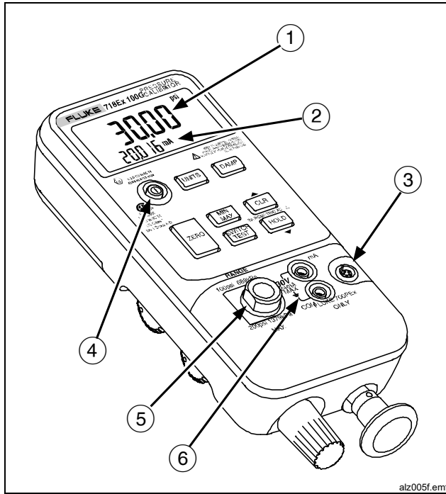
Figure 2. Front-Panel Features
