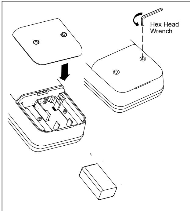
Figure 7. Battery Replacement
